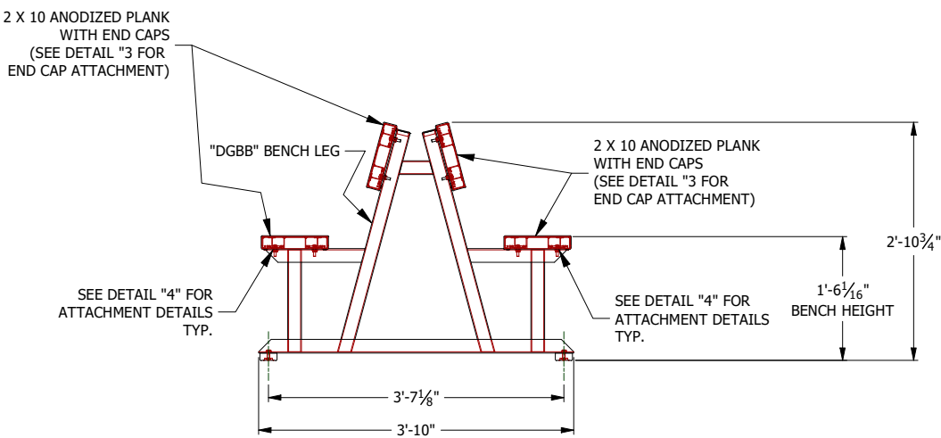
RUBBER FOOT PAD OPTION SEE DETAIL "1"
